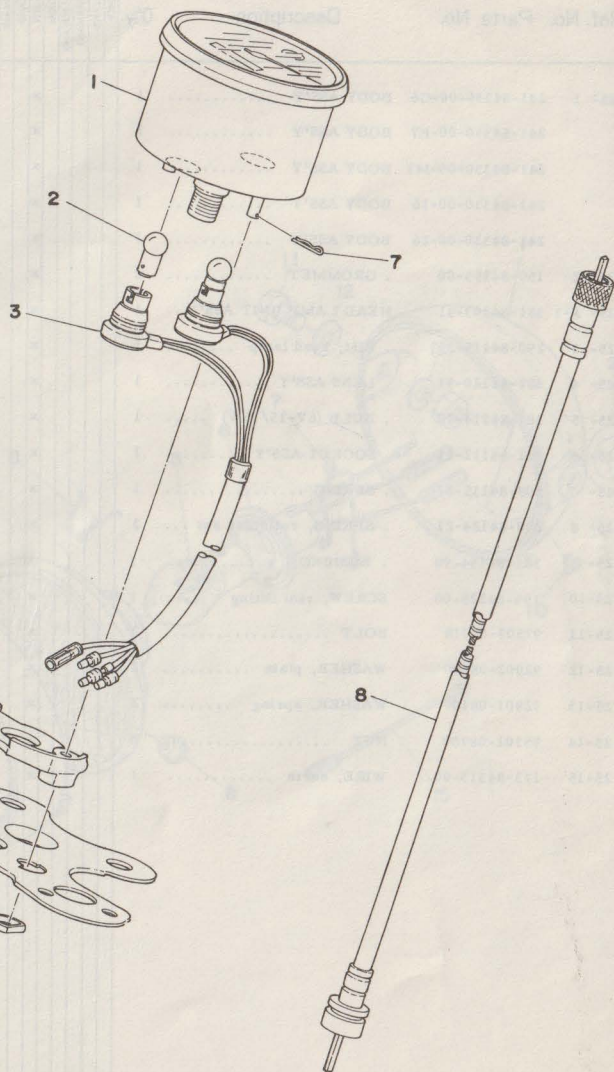
Fig. 26 SPEEDOMETER
