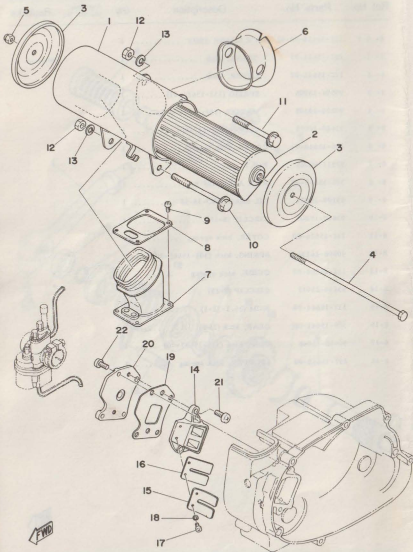
Fig. 9 INTAKE
