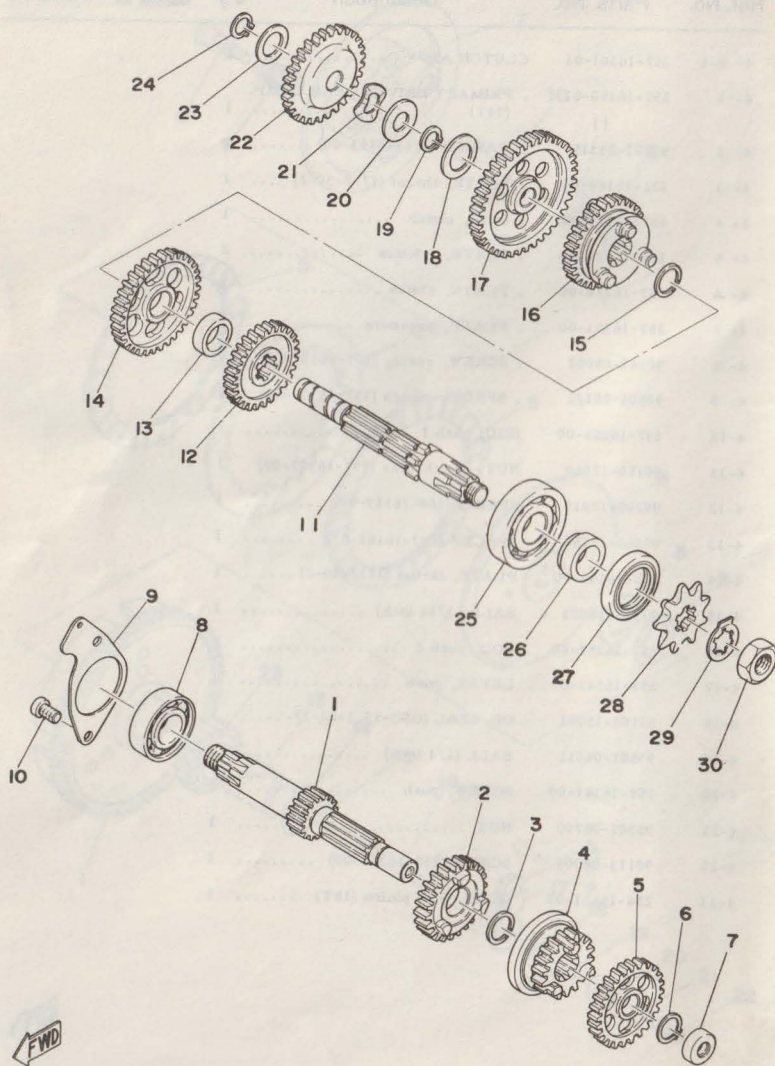
Fig. 5 TRANSMISSION
