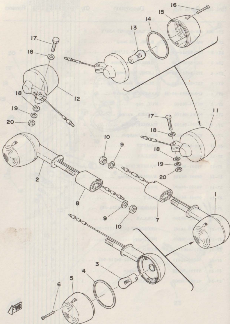
Fig. 28 FLASHER LAMP 1
