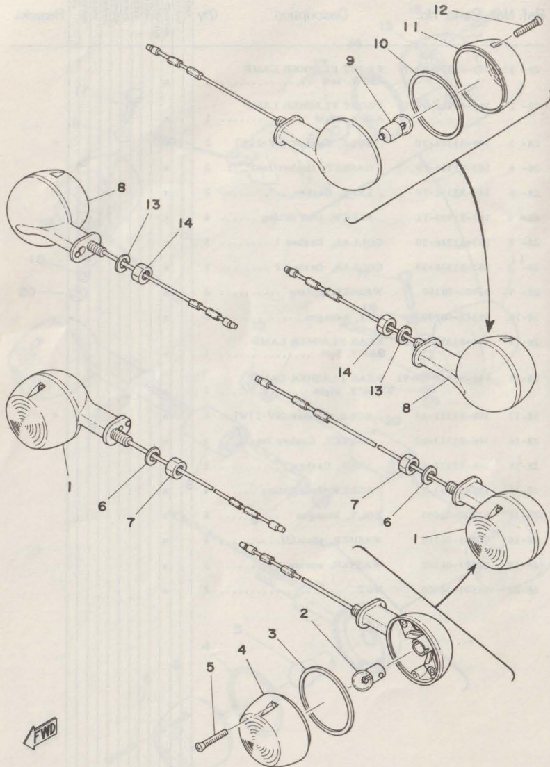
Fig. 29 FLASHER LAMP 2
