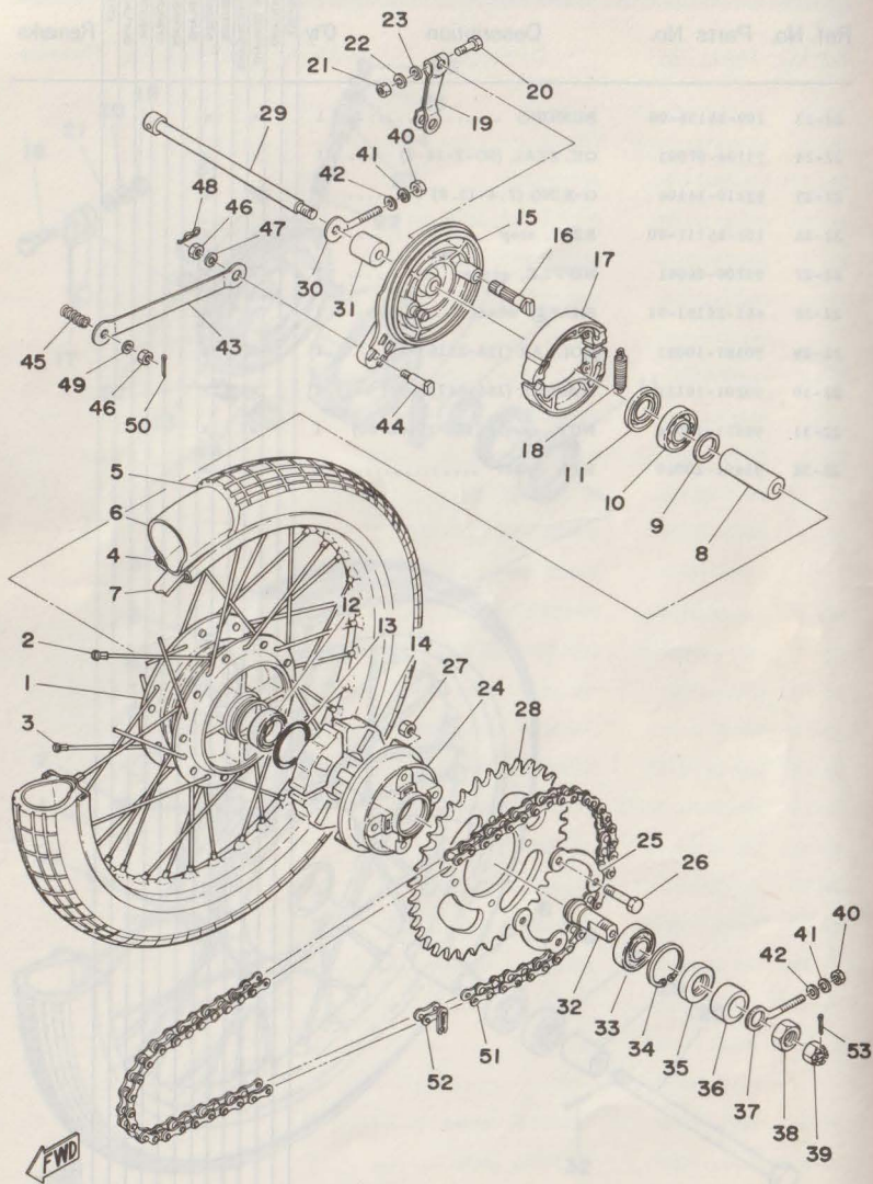
Fig. 23 REAR WHEEL
