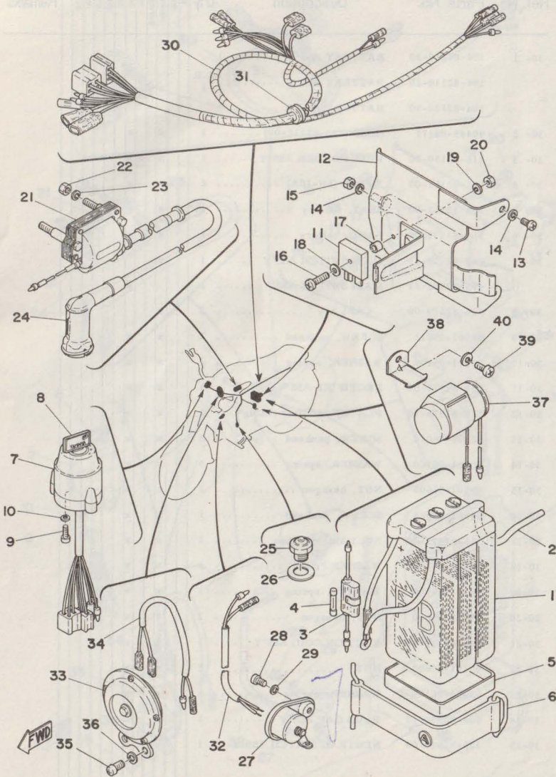
Fig. 30 ELECTRICAL
