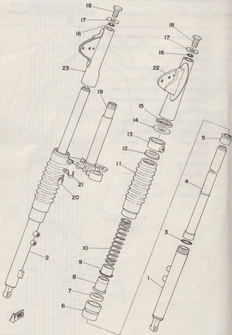
Fig. 17 FRONT FORK
