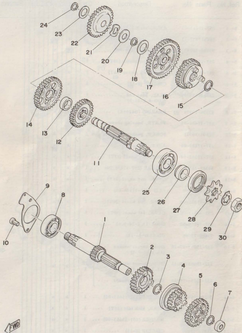
Fig. 5 TRANSMISSION
