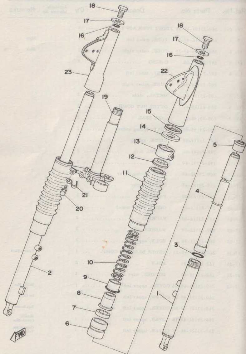
Fig. 17 FRONT FORK
