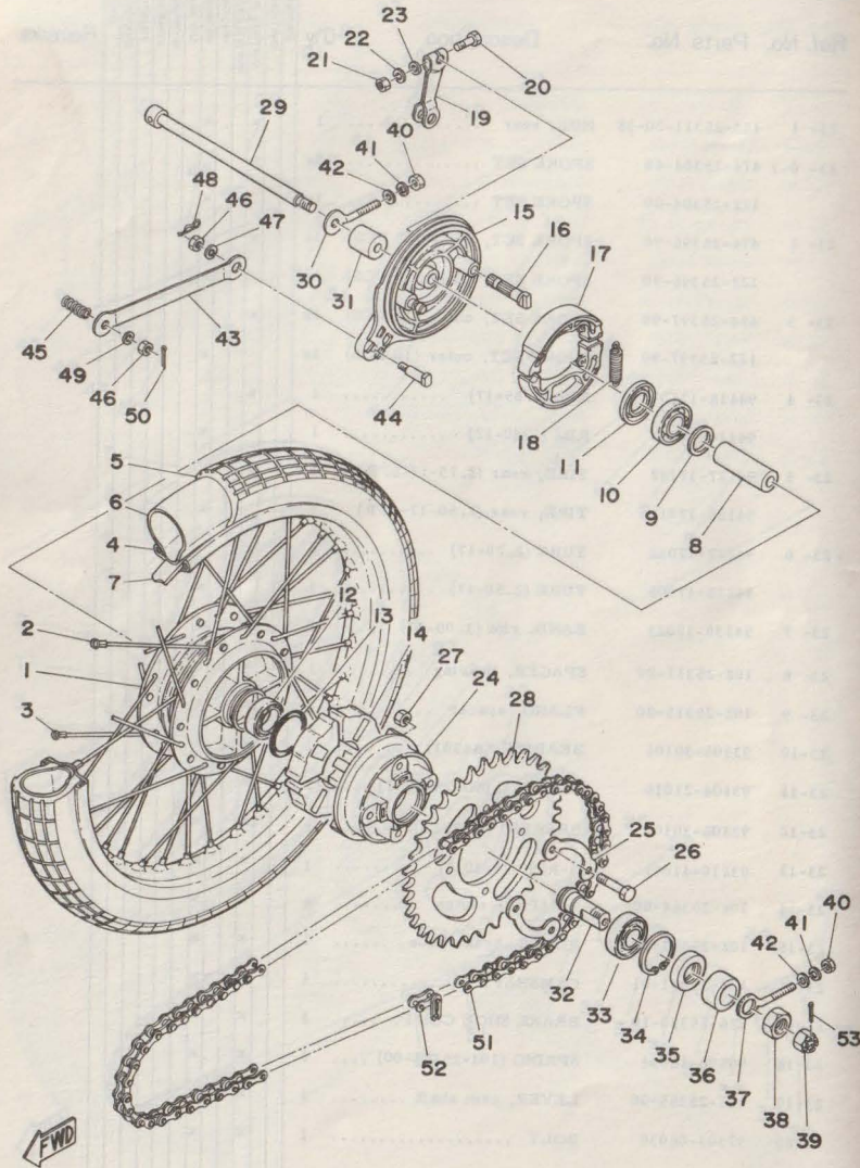
Fig. 23 REAR WHEEL
