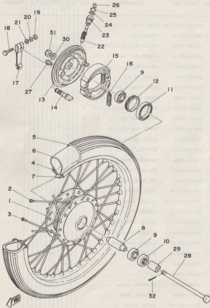
Fig. 22 FRONT WHEEL
